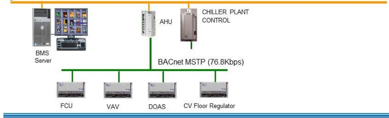
Figure 1: BACnet/IP 10/100MB
