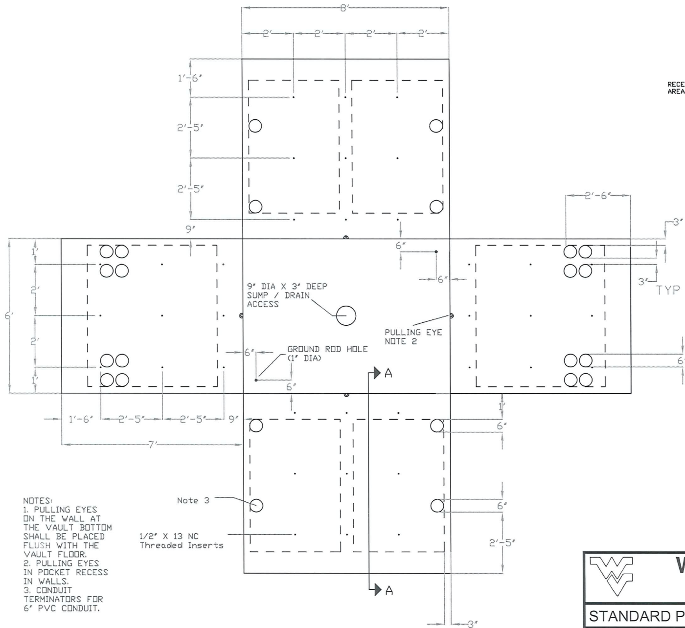
6' X 8' X 7' H.T. PRECAST CONCRETE MANHOLE BASE
